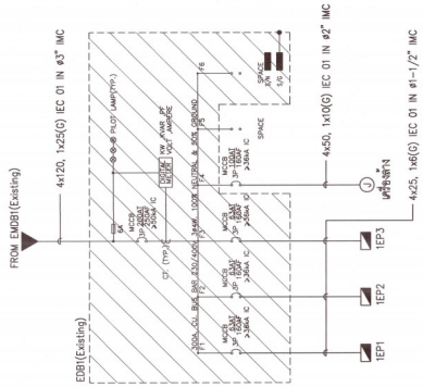
EMERGENCY DISTRIBUTION BOARD (EDB1)
