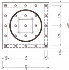
PLAN-TOP SLAB REINFORCEMENT
