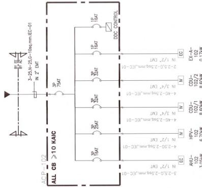
SINGLE LINE DIAGRAM "ACP-102"
